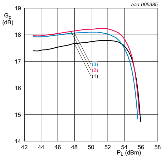
V_{DS} = 28\text{ V}; I_{DQ} = 2400\text{ mA}; t_p = 100\text{ }\mu\text{s}; \delta = 10\text{ }\% . (1) f = 2110\text{ MHz} (2) f = 2140\text{ MHz} (3) f = 2170\text{ MHz}
